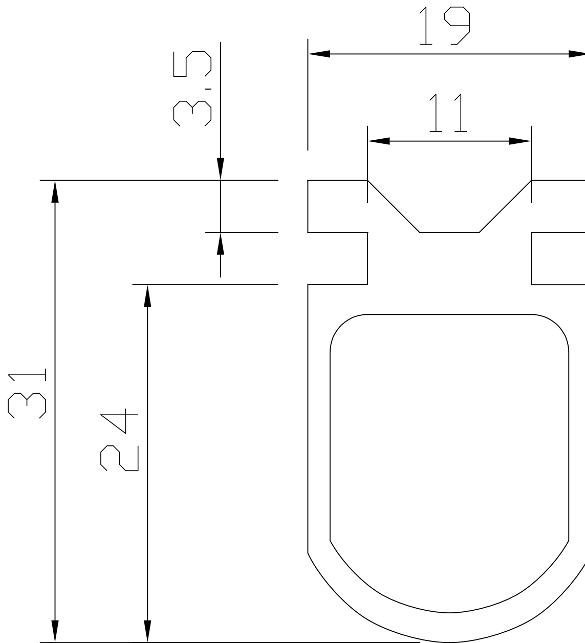
RUBBER SAFETY SEAL (To Suit Galvanised and UPVC Carriers)
